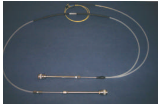
Fig. 4.23: Serial configuration of two porewater pressure sensors
