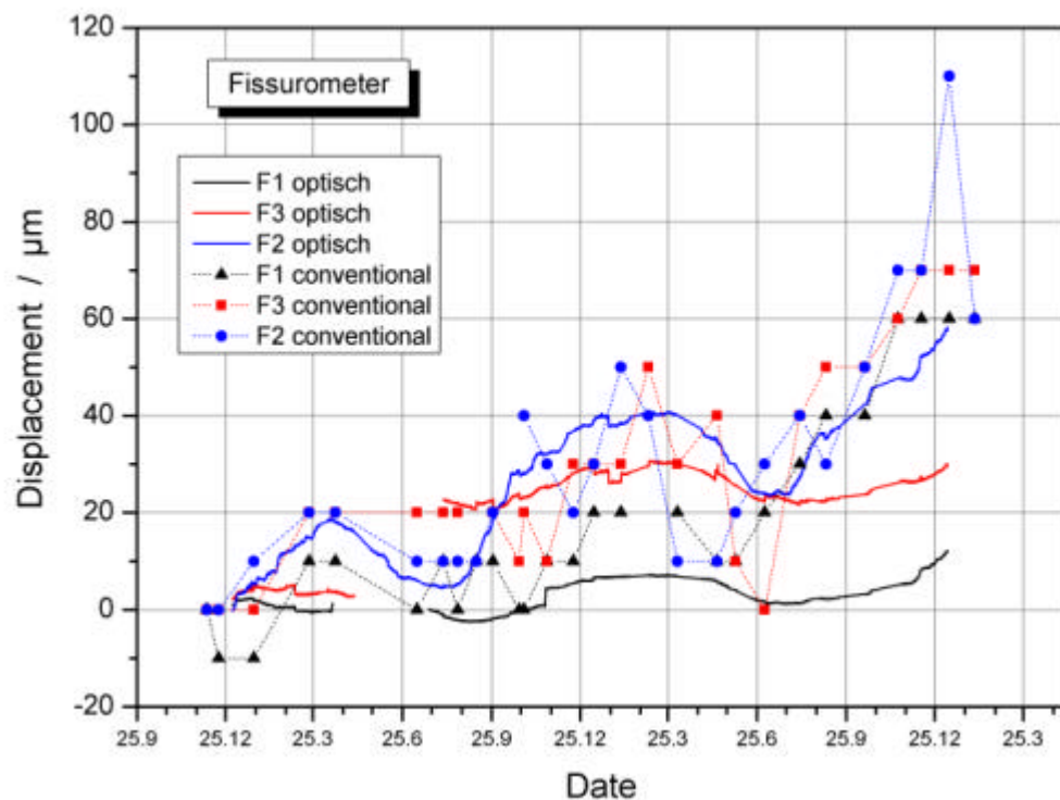
Fig. 4.8: Measurement results of fiber optic and conventional fissurometers at the Morsleben site
