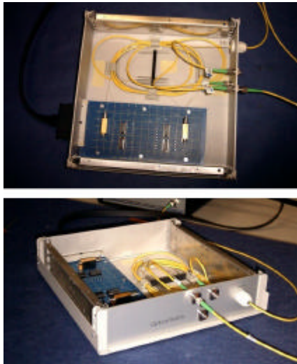
Fig. 5.4: 1x3 optical switch design.
