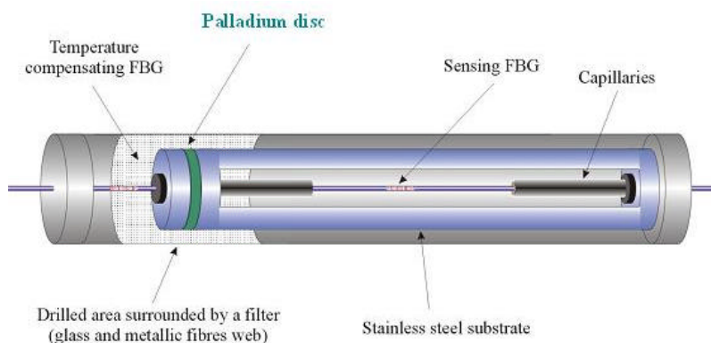
Fig. 4.33: Design of hydrogen sensor I
