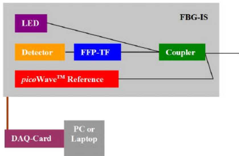
Fig. 5.1: Schematic lay-out of the FBG-IS
