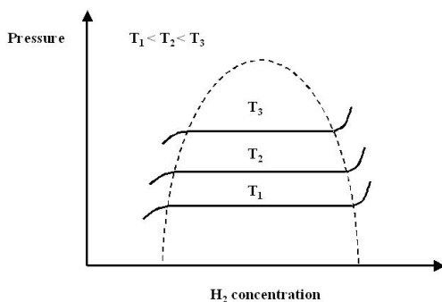
Fig. 4.31: Idealised PCT curves for 3 temperatures
