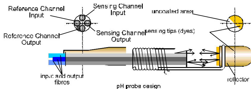
Fig. 4.37: Principle design of pH sensor
