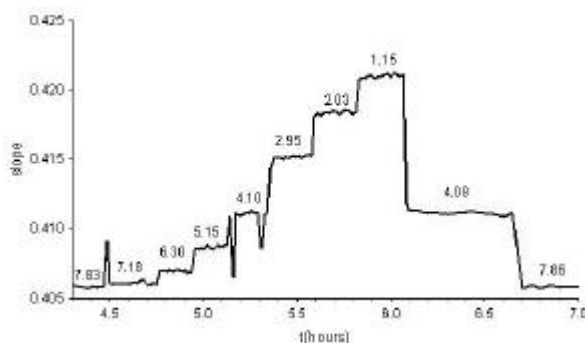
Fig. 4.40: Detail of the temperature characterization at T = 20^\circ\text{C}
