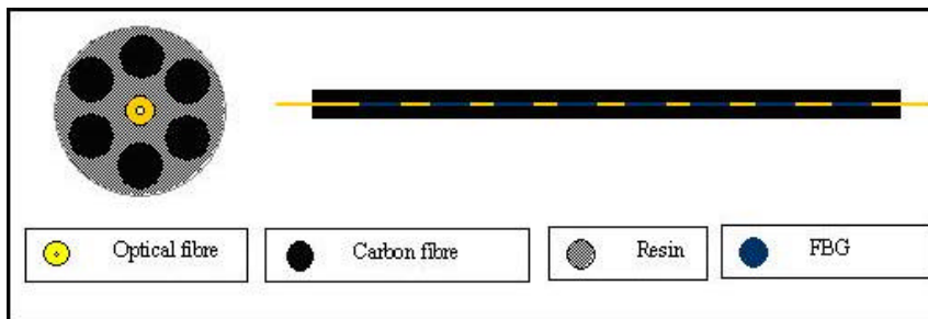
Fig. 4.1: Design of temperature cable
