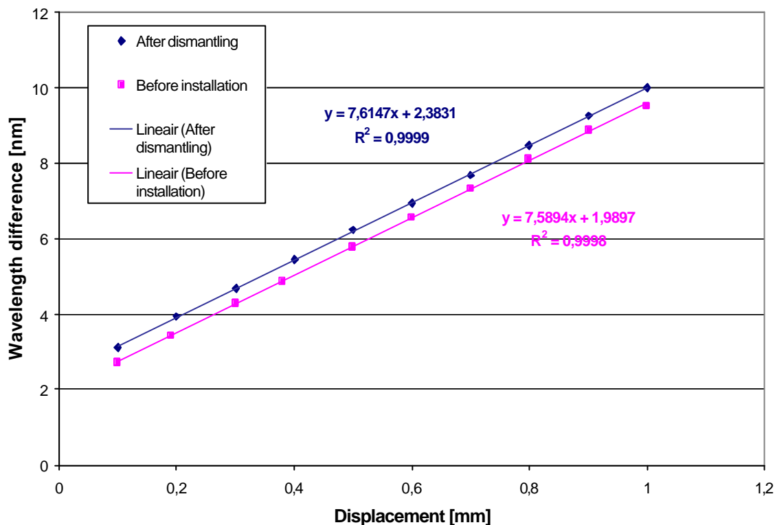
Fig. 4.9: Comparison of sensor calibration before and after the in-situ test
