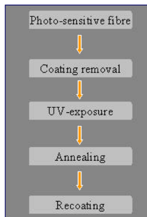
Fig. 5.6: Process steps mechanical gratings
