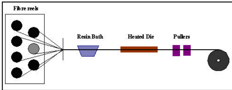
Fig. 4.3: Schematic overview of pultrusion process
