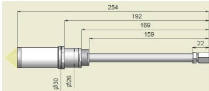
Fig. 4.18: Dimensions of a pore water pressure sensor
