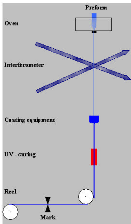
Fig. 5.9: Tower grating production set-up
