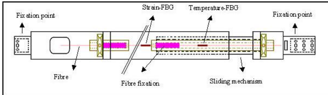
Fig. 4.10: Schematic drawing of an opto-mechanical cell
