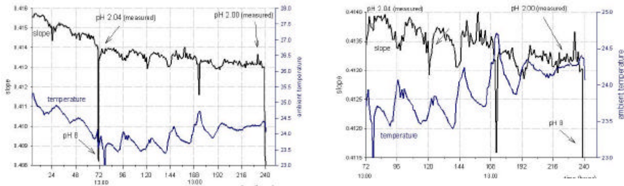
Fig. 4.39: Drift and temperature dependence of the probe characterized with the new opto-electronic unit
