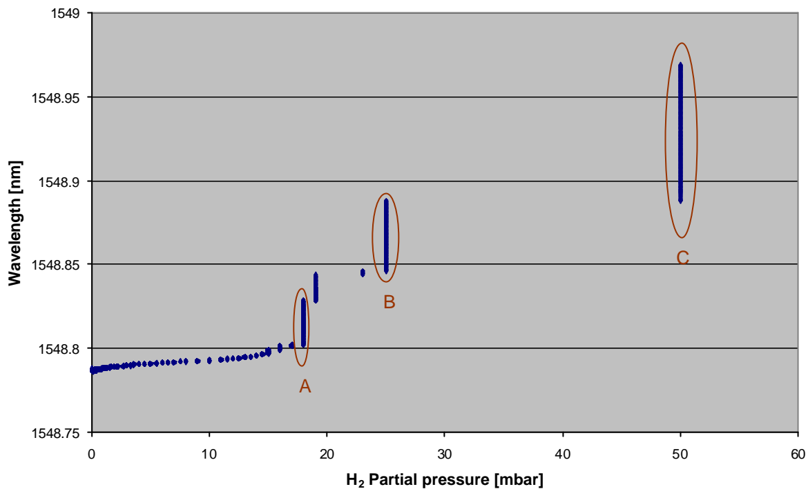
Fig. 4.36: Response of sensor II
