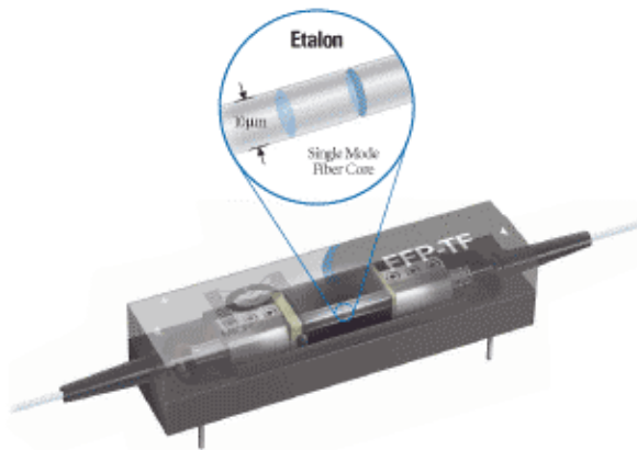
Fig. 5.2: Schematic design of FFP-TF
